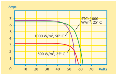
Chart applies to SCHOTT ASE 300 W module only.
